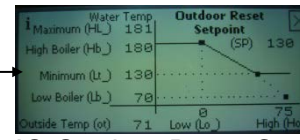
IQ Outdoor Reset Card
